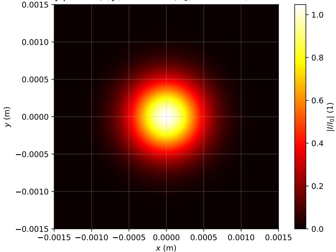
Intensity profile I(x, y, z = 0.398m)/I_0 , P_{in}=0.6P_{cr} , artificial time
